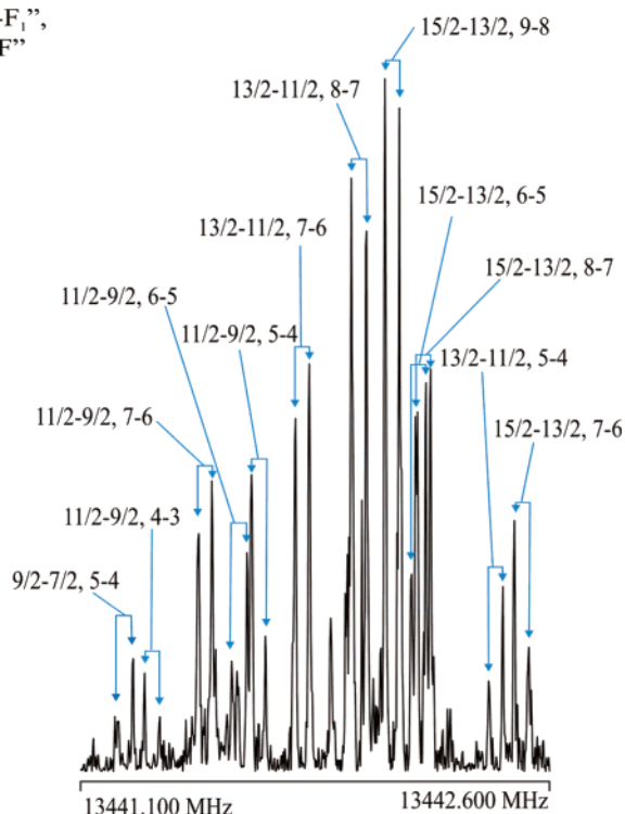
Figure 3. Portion of the observed hyperfine structure in the J = 6-5 transition of ^{131}\text{Xe}^{63}\text{CuF} . A total of 25 250 averaging cycles was taken over 4K data points; 8K transform was used. Quantum numbers F_1'-F_1'' , F'-F'' from coupling scheme \mathbf{J} + \mathbf{I}_{\text{Xe}} = \mathbf{F}_1 , \mathbf{F}_1 + \mathbf{I}_{\text{Cu}} = \mathbf{F} .
